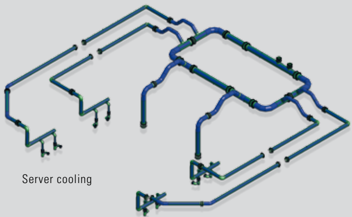
... aquatherm manifold construction.
