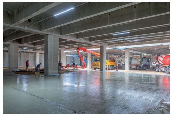
On the ground floor the centerpiece arises: the pipe production
